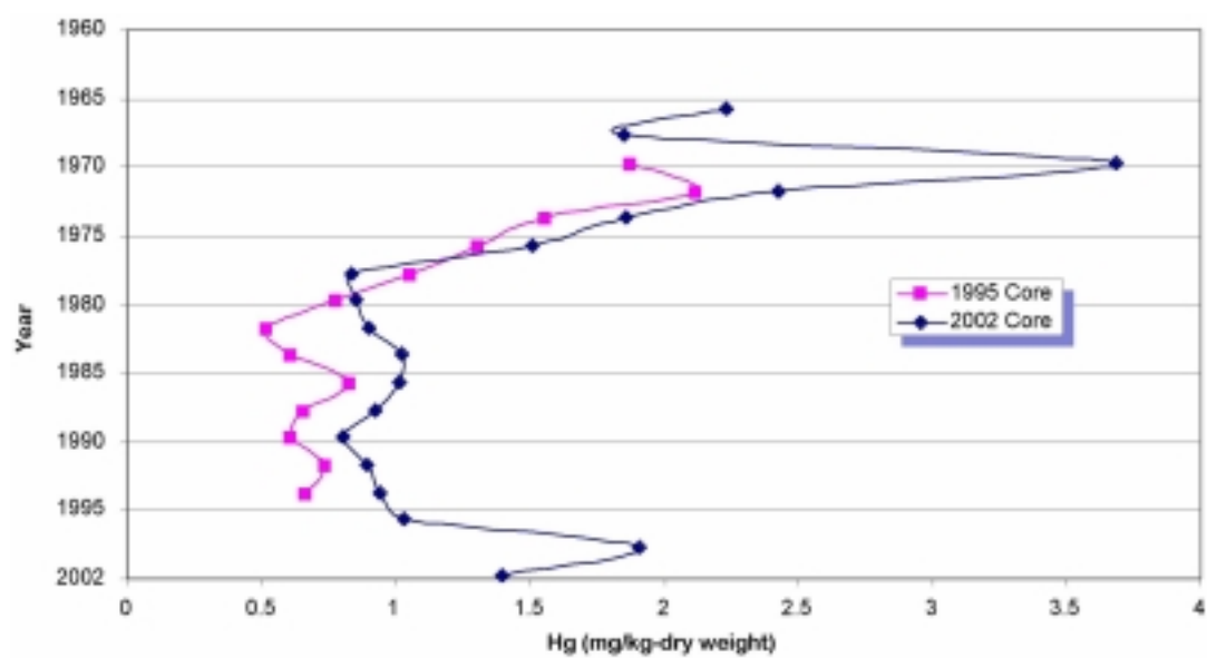
Figure 4: Profile of Mercury Concentrations in Core Samples
