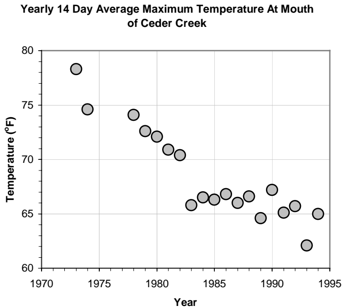
Figure 11. Yearly 14 day maximum stream temperatures at the mouth of Cedar Creek (data provided by Michael Jones in conjunction with the Umpqua National Forest).
