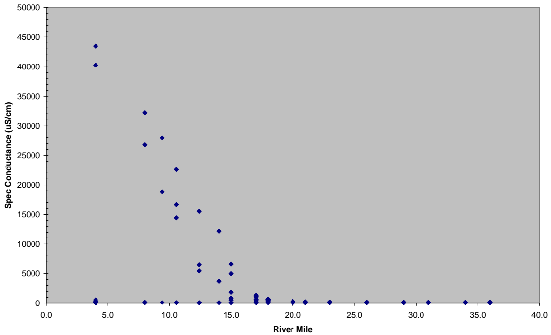
Figure 6: Coquille River Conductivity
