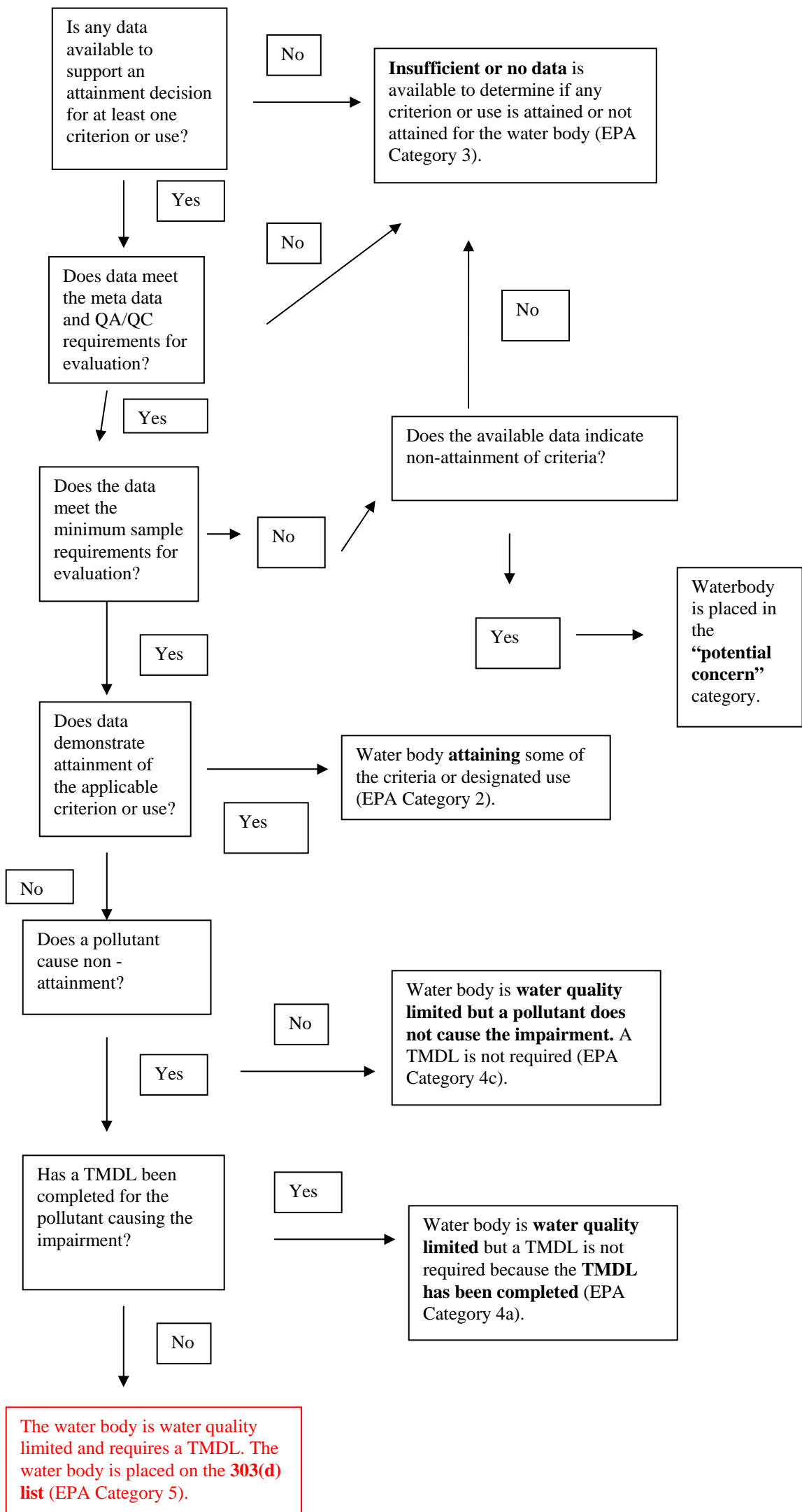
Figure 3: Integrated Report Categories
