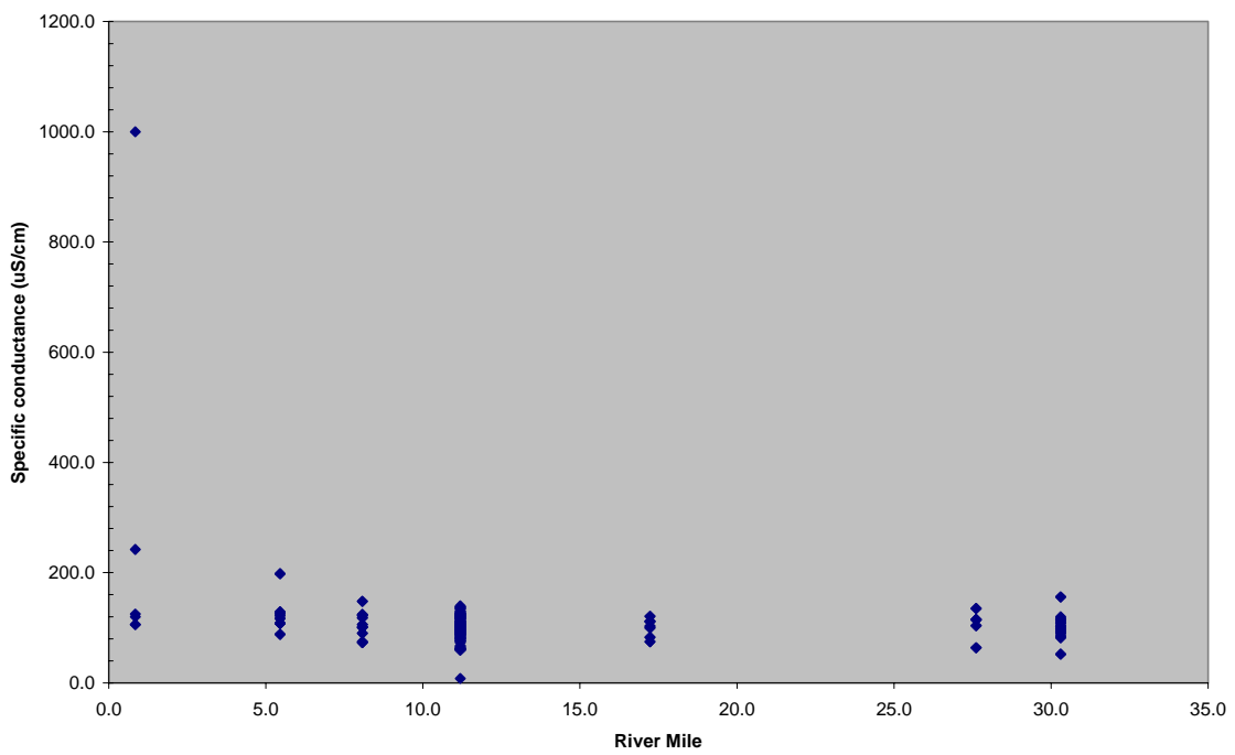
Figure 5: Rogue River Conductivity
