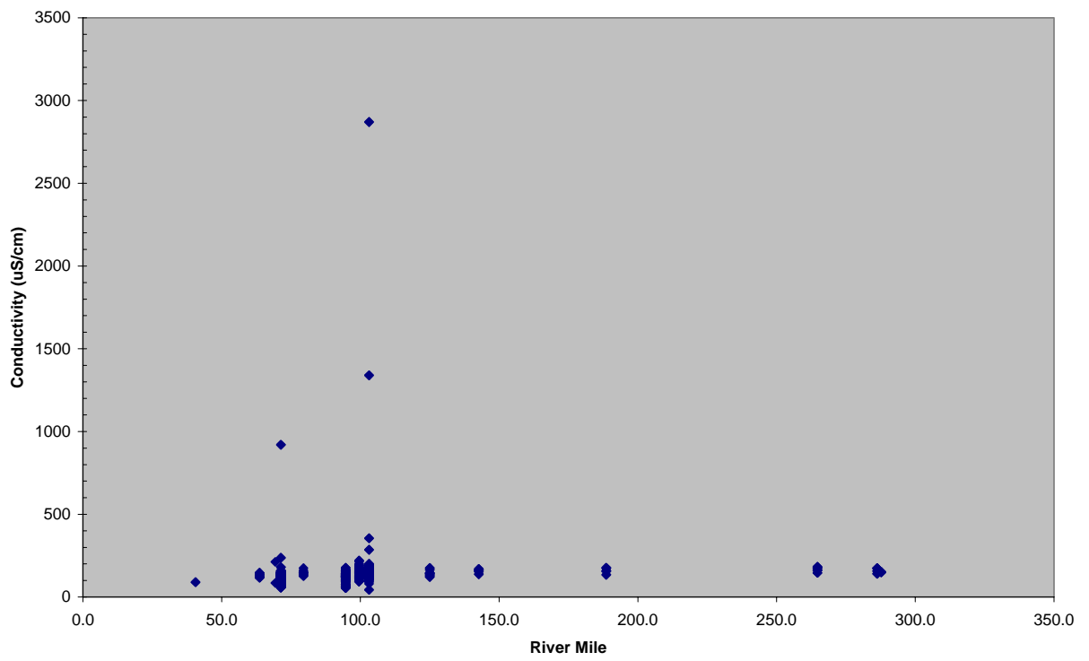
Figure 4: Columbia River Conductivity
