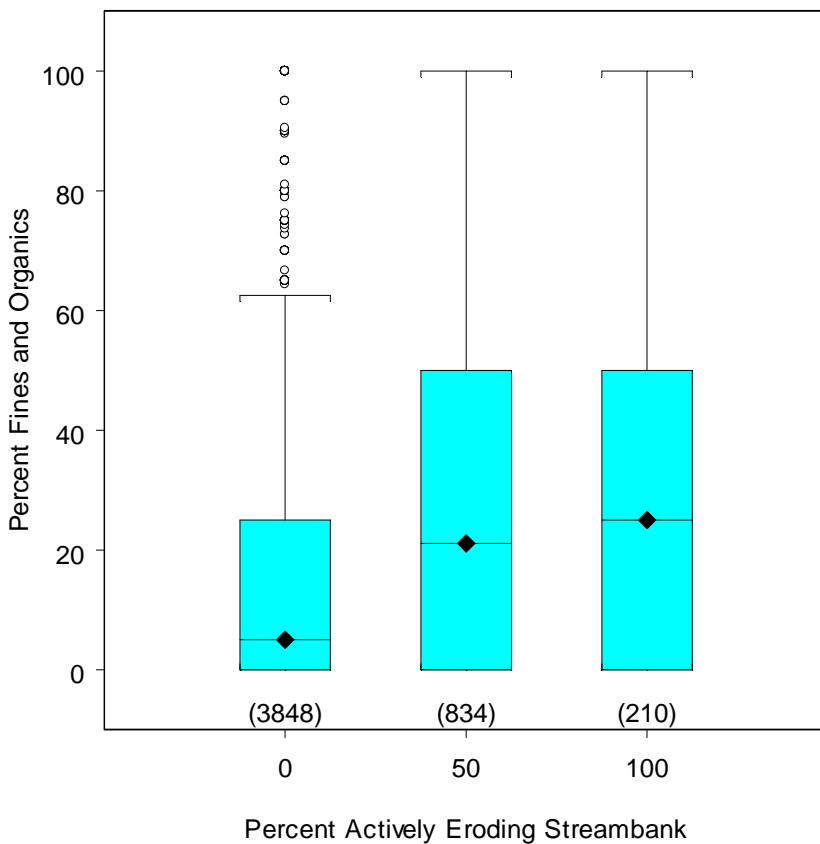
Figure 8: Percent of silt and organics versus percent actively eroding stream bank the surveyed stream in the Wallowa Subbasin. Above data set used the entire Wallowa subbasin and all unit types (i.e. pools through cascades). Sediment data is from the ODFW habitat survey collected between 10/21/1991 and 7/23/1996 in the Wallowa Subbasin.
