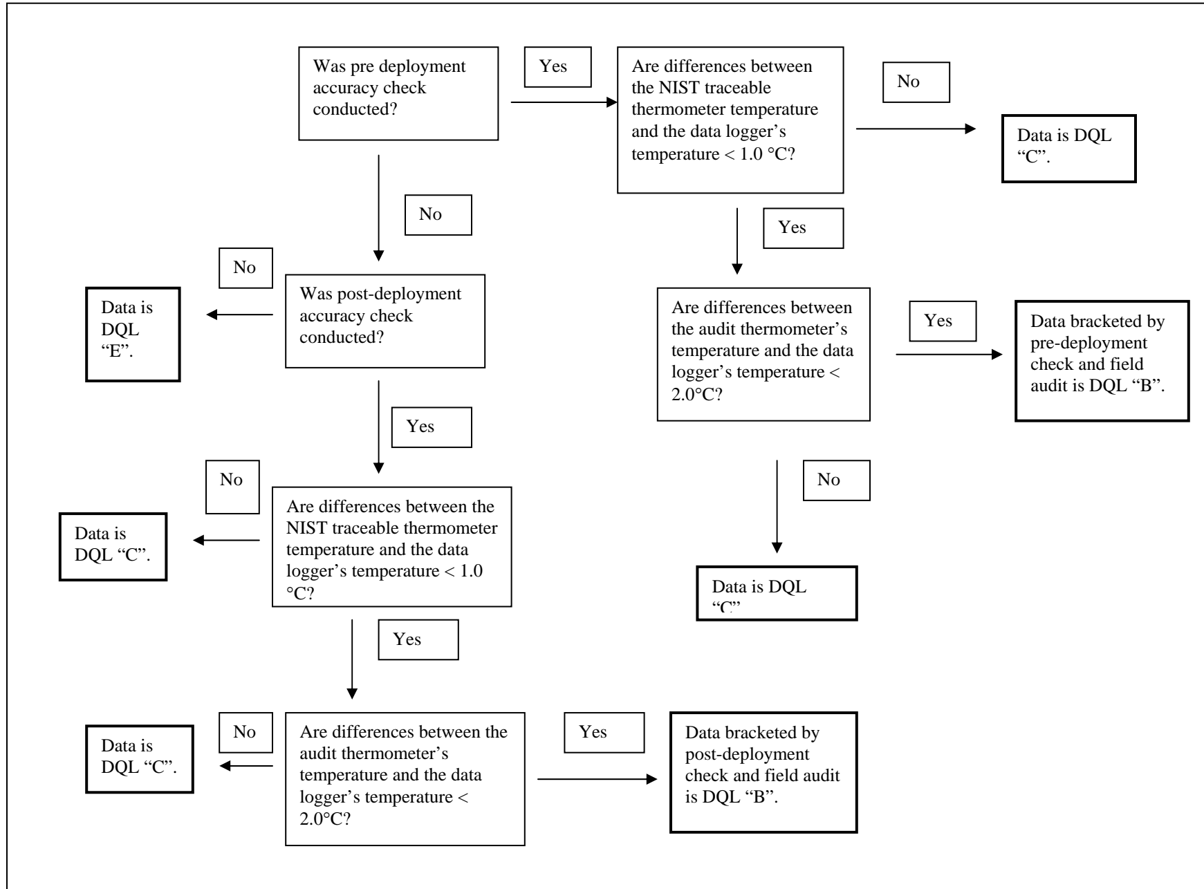
Figure 2: Continuous Temperature Data Grading for Analyses with Pre- or Post- Deployment Accuracy Checks and One (1) Field Audit:
