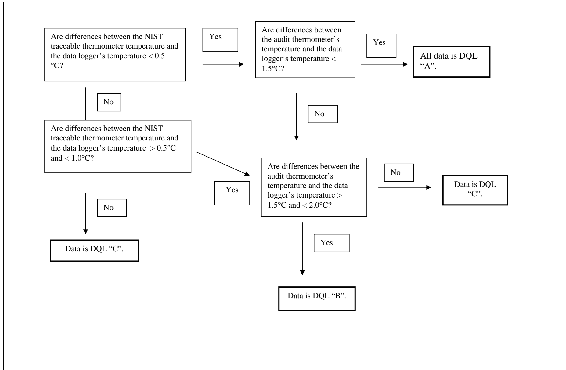
Figure 1: Continuous Temperature Data Grading for Analyses with Pre- and Post- Deployment Accuracy Checks and a Minimum of 2 Field Audits:
