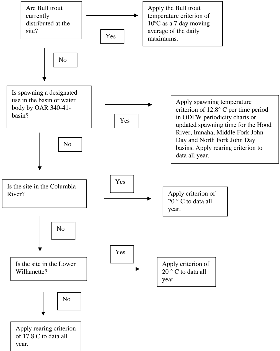
Figure 9: Temperature Data Evaluation
