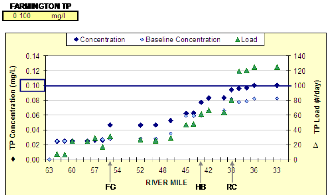
Figure 3-7. Primary TP Mass Balance Results (Median TP Concentration, May through October, 2002-2007) Assumes TP Mass Load ≤ 66.1 lb/day, current flow augmentation levels, and tributaries meeting water quality standards.(See Appendix B-1, Exhibit 2-10). Baseline Total P concentration (◊ light blue diamond) reflects current river concentrations, while the Concentration (◊, dark blue diamond) and load (△ green triangle) are projected future conditions based on a future 66.1 lb./day load.
