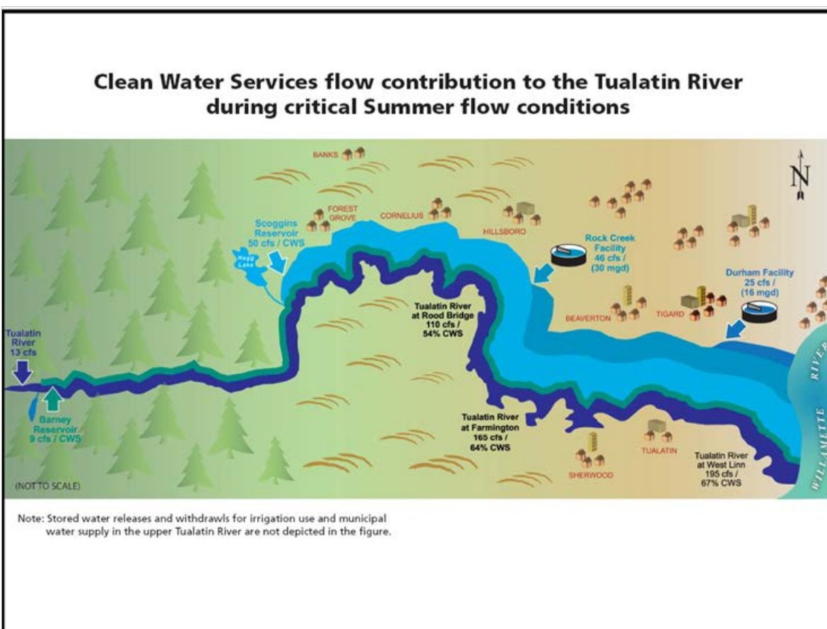
Figure 1-3. A schematic that shows the relative flow contributions to summer low flow in the mainstem Tualatin River from Clean Water Services flow augmentation program, and Waste Water Treatment Facility discharges.
