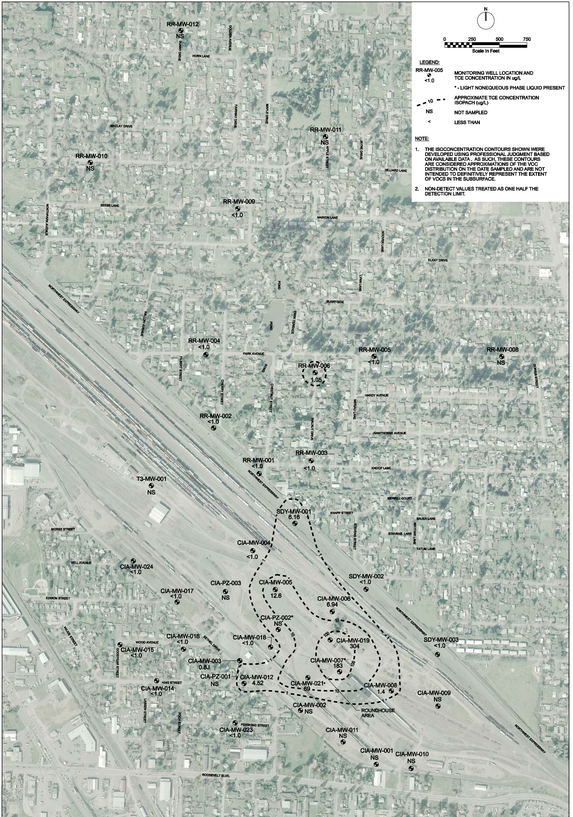
FIGURE 6 TRICHLOROETHENE CONCENTRATION CONTOURS - APRIL 2009 SHALLOW ZONE UNION PACIFIC RAILROAD COMPANY EUGENE, OREGON - ACTIVE SP YARD
