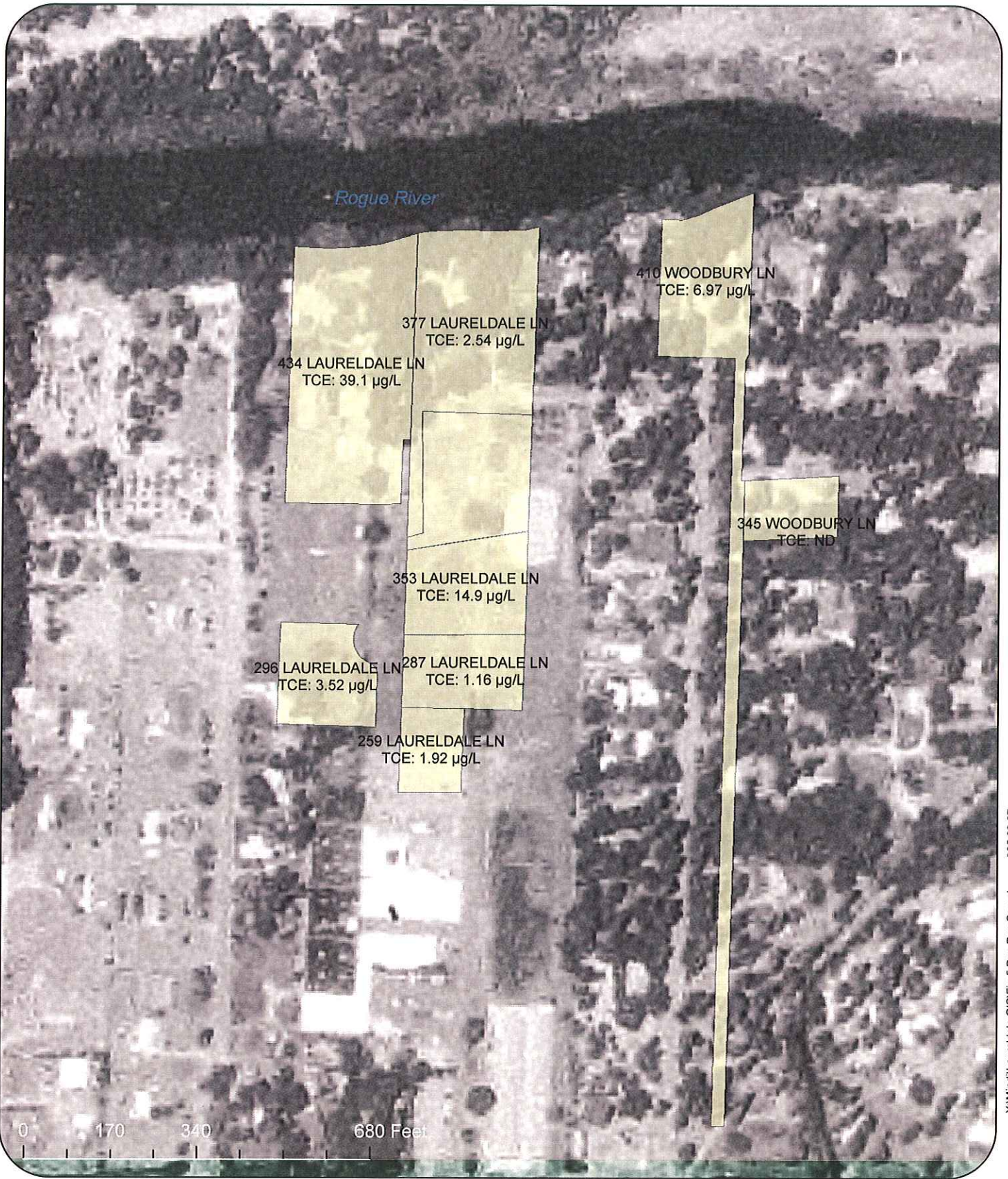
Figure 5 Domestic Well Sampling Results December 2006 and January 2007 Laureldale Lane Groundwater Study Area XPA
