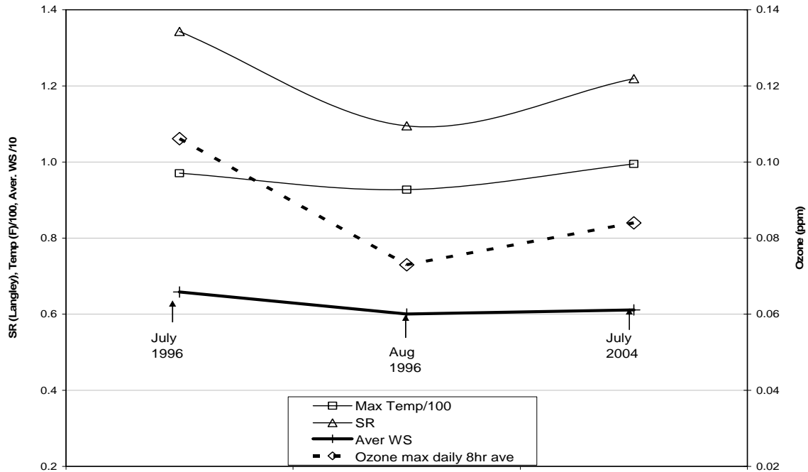
Figure 15: Three day episodes with maximum temperatures \geq 90^{\circ}\text{F} , wind speed < 10\text{mph} , Solar Radiation >1 Langley/hr with third day on Saturday 9 .
