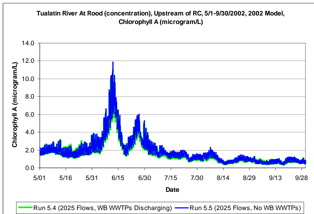
Figure 4-2. Chlorophyll a at Rood Road. Exhibit 3-3 shows results for chlorophyll a at Rood Road because that is the downstream-most location for the Upper River and therefore expected to show the maximum potential effect on algal growth by discharges to the Upper River.
