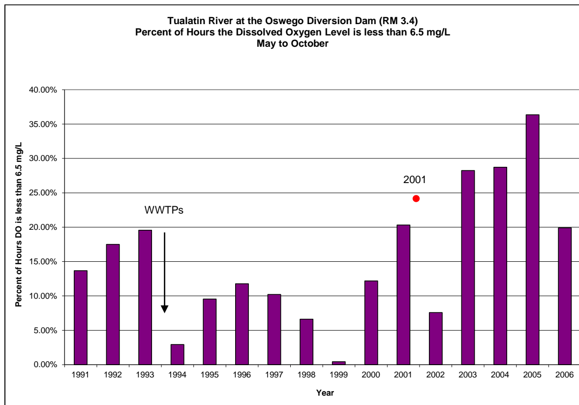
Figure 4-4. The percent of hours in each TMDL season that dissolved oxygen levels were less than 6.5 mg/L at the Oswego Dam at River Mile 3.4 in the Lower Tualatin River.
