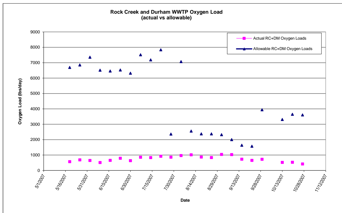
Figure 4-3. The allowable oxygen-demand and the actual oxygen demand for Clean Water Services Rock Creek and Durham Treatment Plants during the TMDL season of 2007. The Y-axis shows the pounds per day of actual and allowable (2005 Watershed Permit) oxygen-demanding substances in discharged water (CBOD + NBOD).
