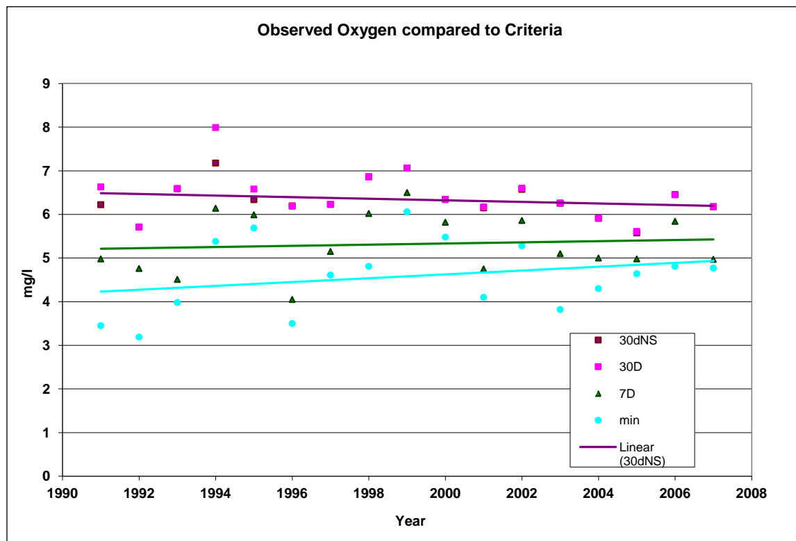
Figure 4-5. Observed values for various dissolved oxygen statistics at the Oswego Dam site (RM 3.4) from 1990-2007.
